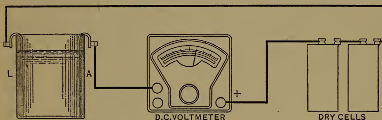
FIG. 19.—TESTING A NODON VALVE WITH DRY CELLS.
